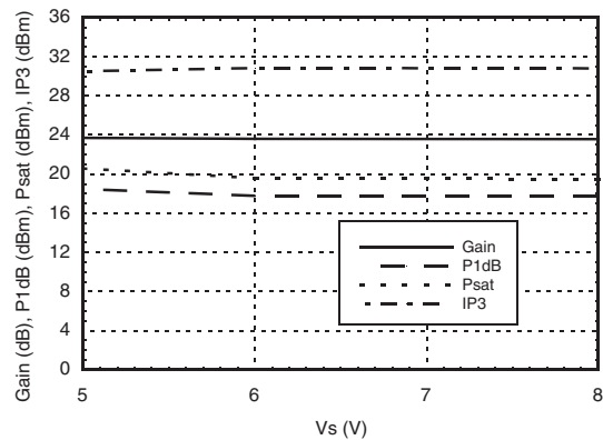
Gain, Power & Output IP3 vs. Supply Voltage for Constant I_{cc} = 62 \text{ mA} @ 850 MHz
