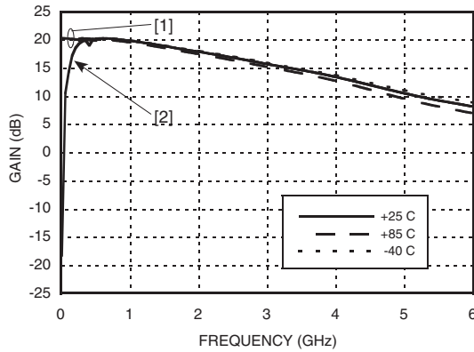
Maximum Gain vs. Frequency
